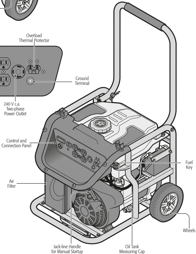
Control and Connection Panel
