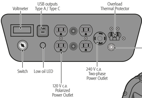
Control and Connection Panel
