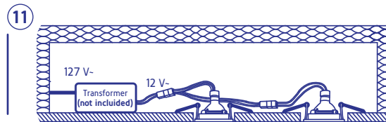
Diagram to install a 12 V~ lamp
