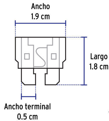
Fusible standard
